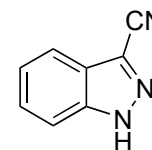
1H-indazole-3-carbonitrile (1) 13 C NMR (125 MHz, CDCl 3 )
